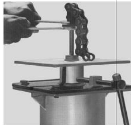
9. Place Third plate on Rod vice, take off the Chain support and remove the Chain assembly
