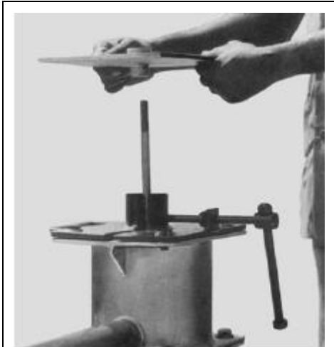
10 Unscrew check nut and remove Third plate assembly
