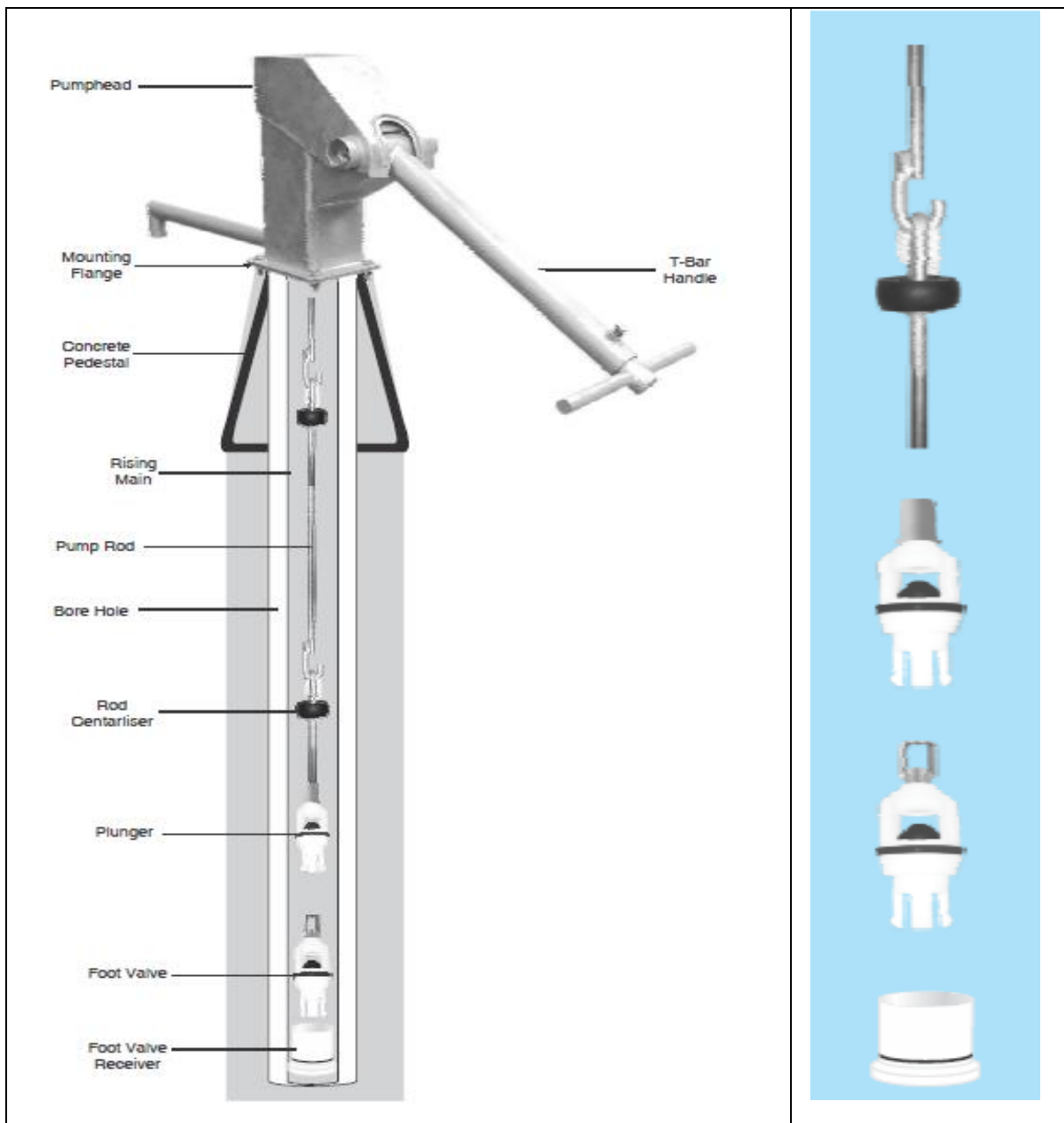
Figure 3-7: Details of Afridev Hand Pump
